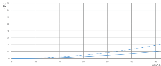
Drukval Ventielcollector 90° [Pa]
