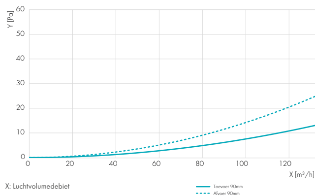
Drukval Ventielcollector 90° [Pa]
