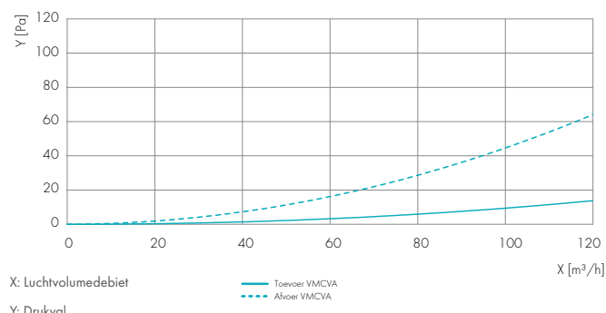
Drukval Wandcollector [Pa] VMCA 90 + NOVAL
