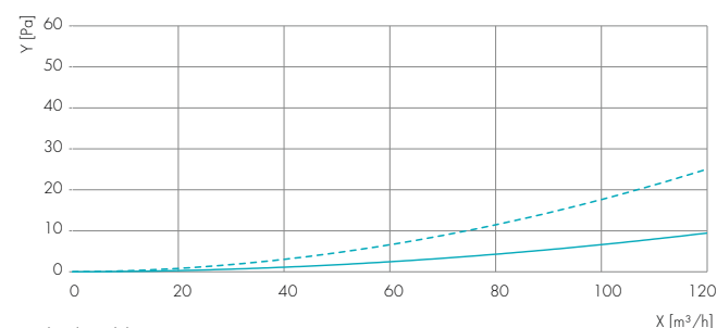
Drukval Wandcollector [Pa] VMCA 290 + NOVAL
